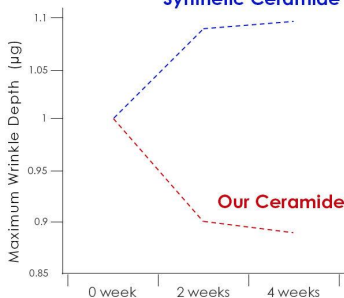
Synthetic Ceramide
